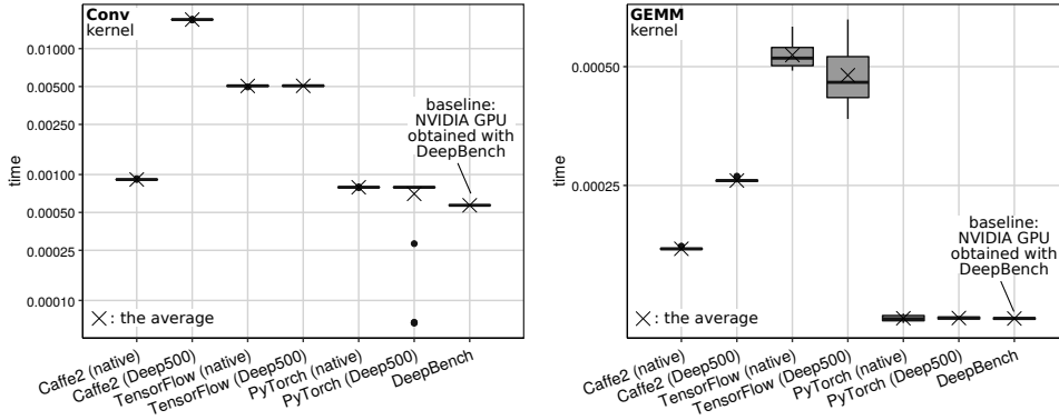
Fig. 7: Analysis of Deep500 Level 0: Performance of one specific convolution (left, N = 16, C = 3, H = W = 224 , filter size 3 \times 3 ) and matrix multiplication (right, M = K = 2560, N = 64 ) parameters from DeepBench.
