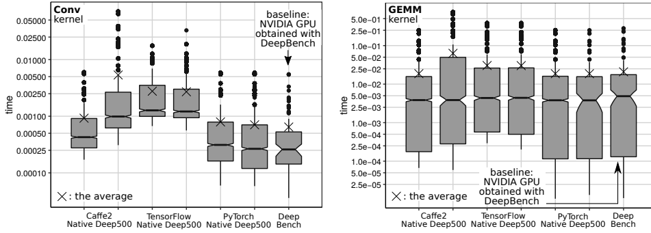
Fig. 6: Analysis of Deep500 Level 0: Performance of operators implemented with Deep500 and selected frameworks, together with the DeepBench baseline.
