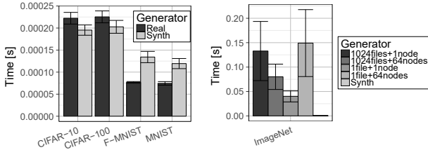
Fig. 9: The latency of loading various datasets.
