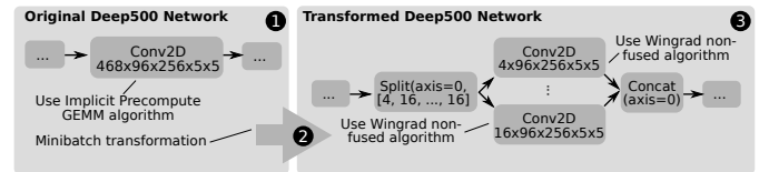
Fig. 8: The illustration of the Microbatch transformation.
