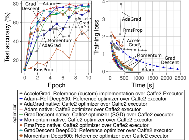
Fig. 10: The analysis of test accuracy vs. epoch number and training loss vs. elapsed time for different optimizers (assuming Caffe2, ResNet-18, CIFAR).
