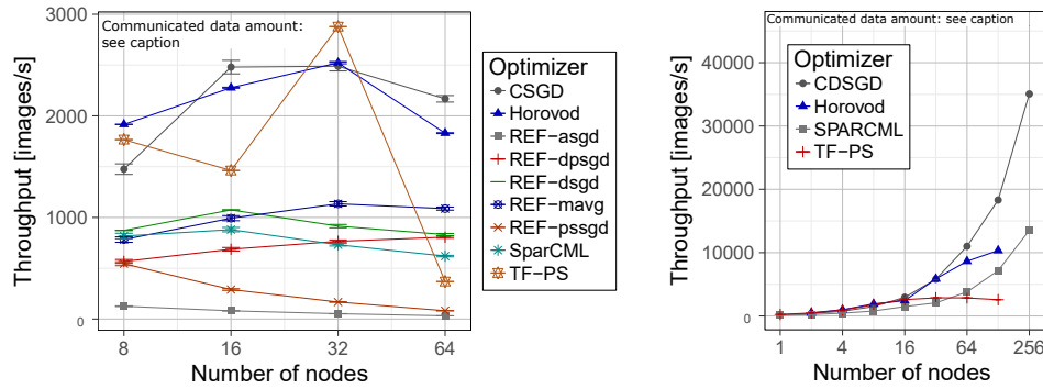
Fig. 13: Scaling of Level 3: Strong (left) and weak (right) scaling on Piz Daint and ImageNet. The amount of communicated data per node: 1,022GB (CDSGD), 1,021GB (SparCML), 1.022GB (REF-dsgd), 30.68GB (REF-asgd), 2.045 (REF-dpsgd) 2.044 (REF-pssgd).
